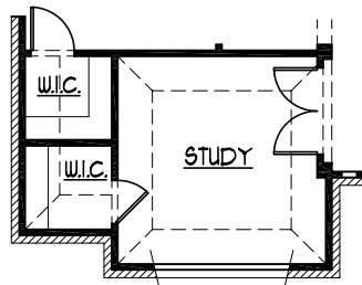
OPT. STUDY A
